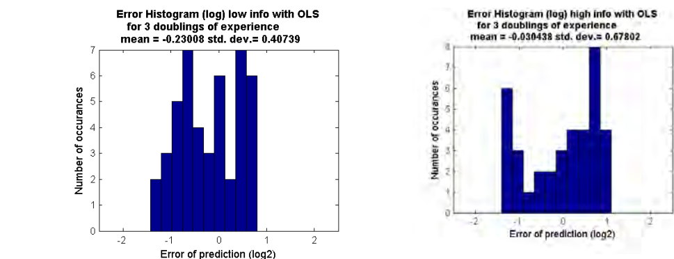
Figure 24 Comparing forecasts made with less and more information
