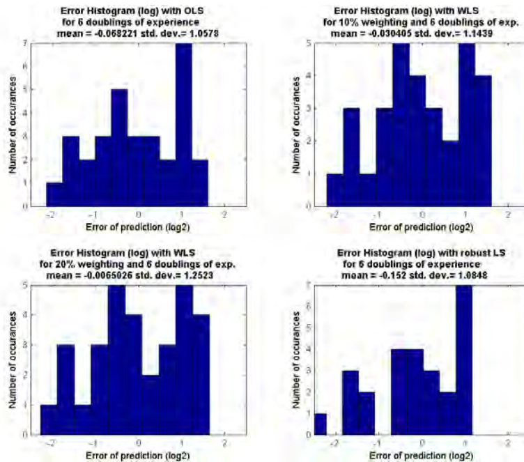
Figure 20 Histogram of the log of the errors for 6 doubling of cumulative experience
