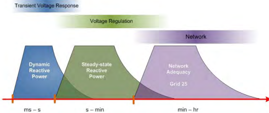
Figure 5: Voltage Control Services (Source: EirGrid)
