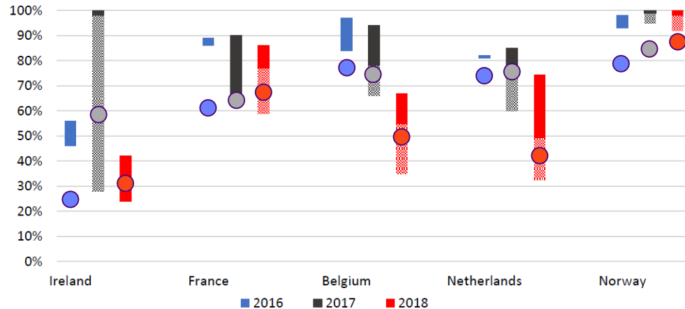
Figure 16: T-4 Forward De-rating Factor Ranges (2018,2017,2016)
