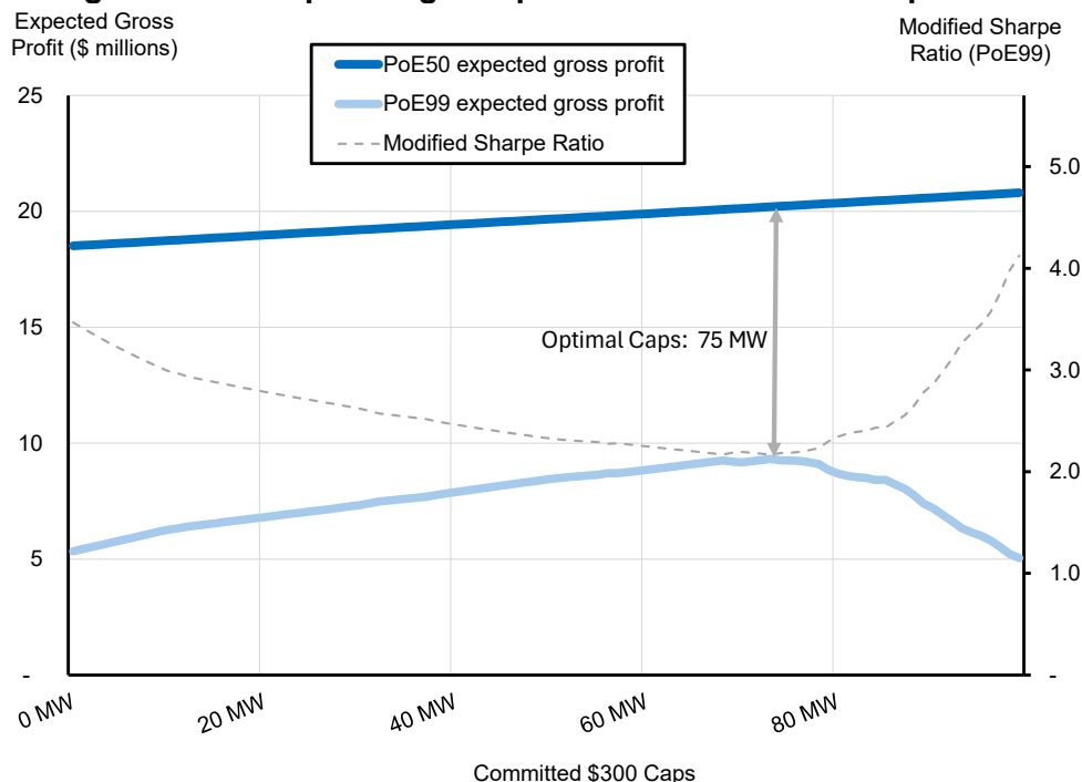
Figure 9: GT expected gross profits and Modified Sharpe Ratio
