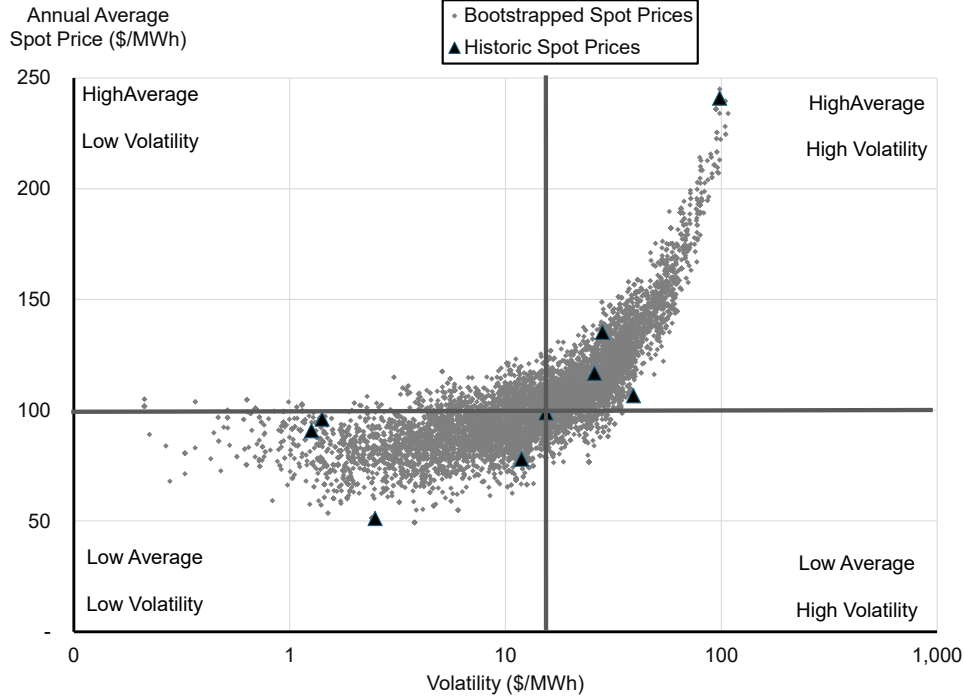
Figure 6: Spot electricity prices
